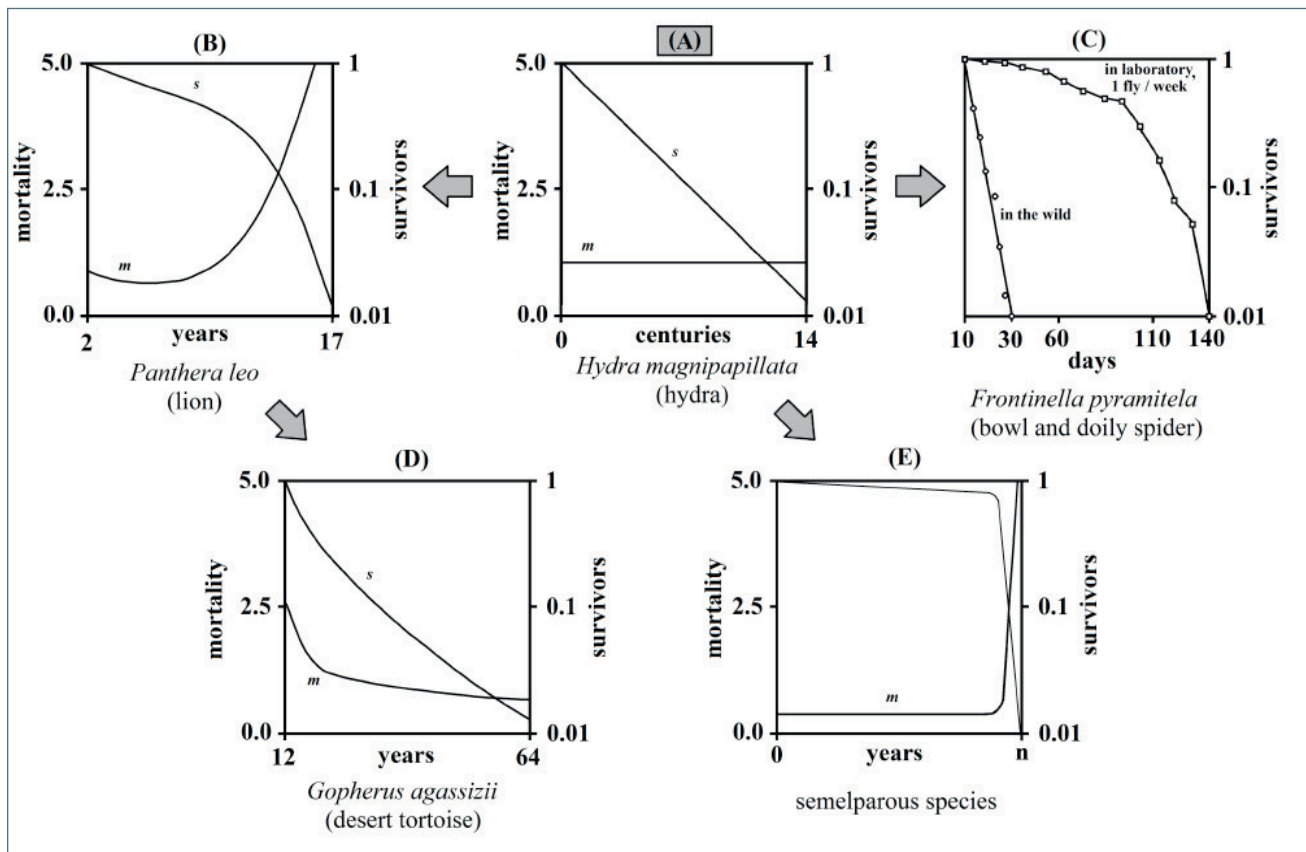
Figure 7B. For the new paradigm, the primary condition is (A) and the other conditions are derived.
