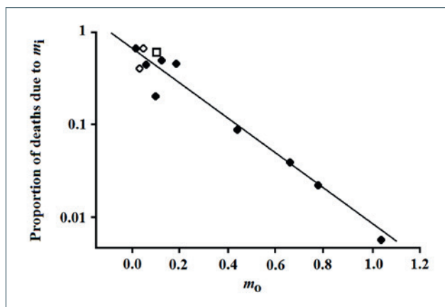
Figure 5. Inverse relationship between m_0 and the proportion of deaths due to m_i . Solid diamonds refer to bird species, open diamonds to mammal species, open square to Homo sapiens ; ordinates are in logarithmic scale. Data for mammals and birds are from Ricklefs, 1998 9 , Table II; data for H. sapiens are from Hill, Hurtado, 1996 10 . Without the data of our species, the linear regression has the following values: r = -.758708 , t = -3.494043 , p < 0.01 (from Libertini, 2008 88 ).
